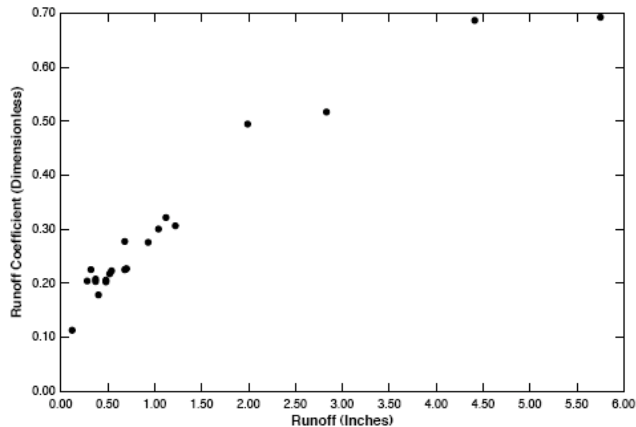
08156800 Shoal Creek at 12th Street Austin Texas TTU Watershed ID 1108
